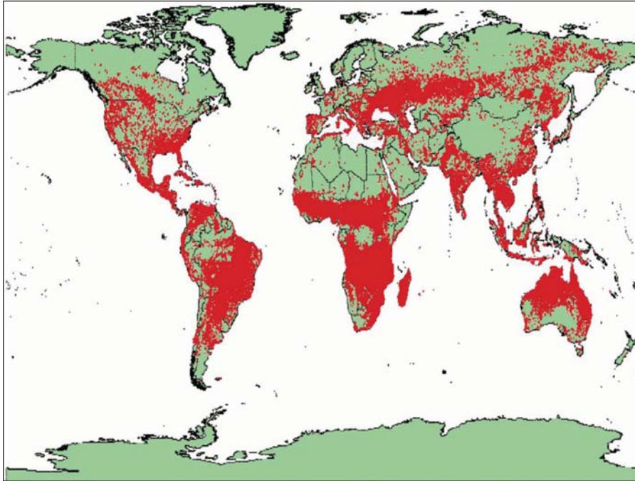
Figure 3 Global cumulative active fire detections (23 April 2001 to 25 February 2002) from the MODIS Land Rapid Response System. Each dot represents a single 1-km MODIS active fire pixel detected during the time period from Justice et al. (2002)
