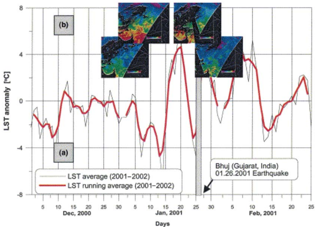
Figure 1 MODIS detection of a land surface temperature anomaly of 4°C 5–6 days before the Bhuj earthquake hit in Gujarat, India 2001. From Ouzounov and Freund (2004)
